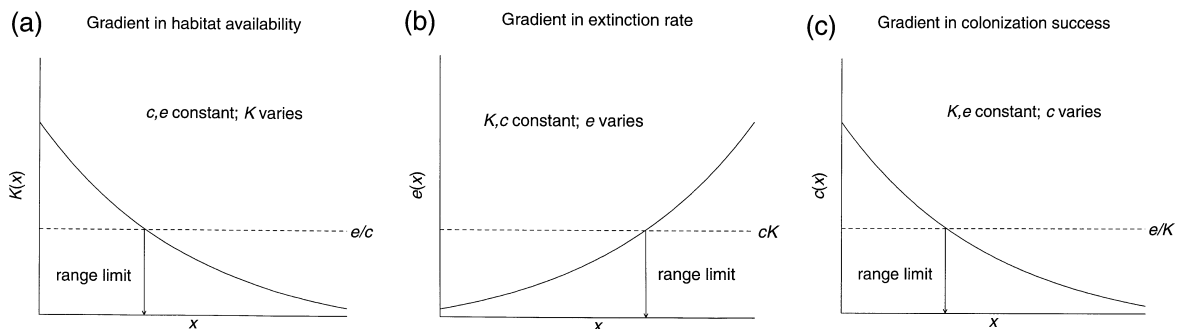
Figure 1 Graphical depiction of three routes to range limits in metapopulations along gradients. (a) Colonization and extinction rates are constant along the gradient, but habitat availability varies. (b) Habitats are uniformly available along gradient, as are colonization rates, but extinction rates increase. (c) Habitats are uniformly available, and extinction rates are constant, but the rate of colonization per habitable, empty patches, per occupied patch, declines. The specific shape of the parameter gradients is arbitrary.
