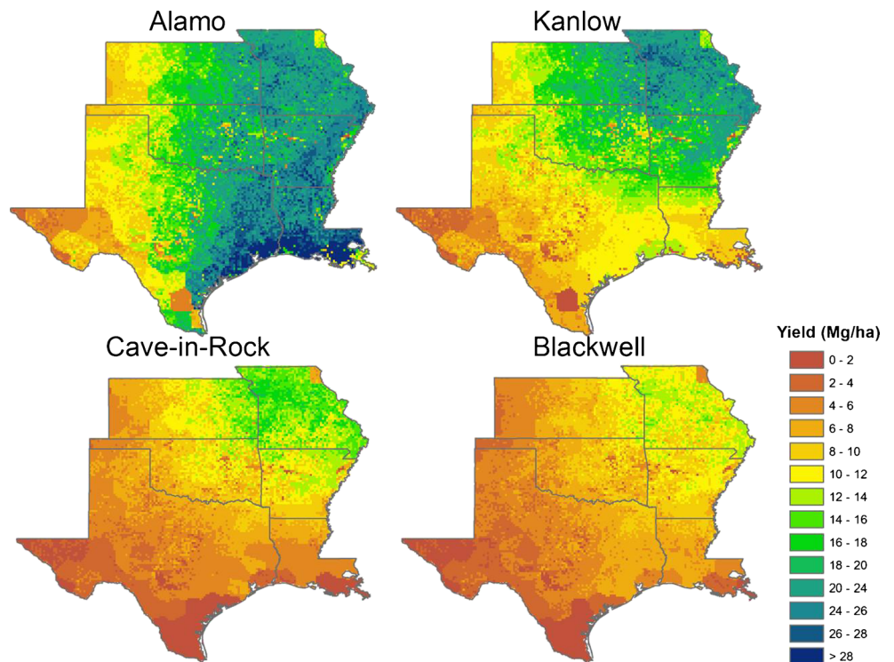
Fig. 3 Spatially continuous yield estimates simulated using the ALMANAC model for four switchgrass cultivars (Alamo, Blackwell, Cave-in-Rock, and Kanlow) in the central and southern Great Plains
